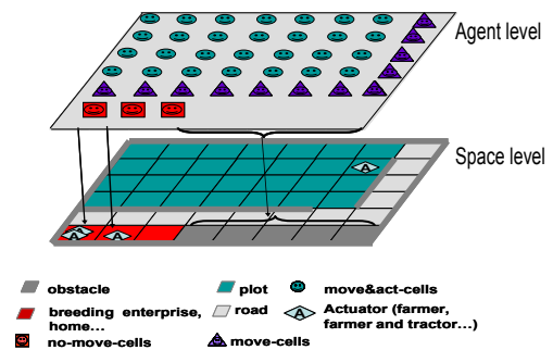
Figure 1. Representation of space as a MAS.
