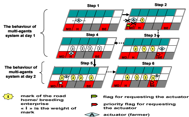
Figure 3. Construction of a mark trail.
